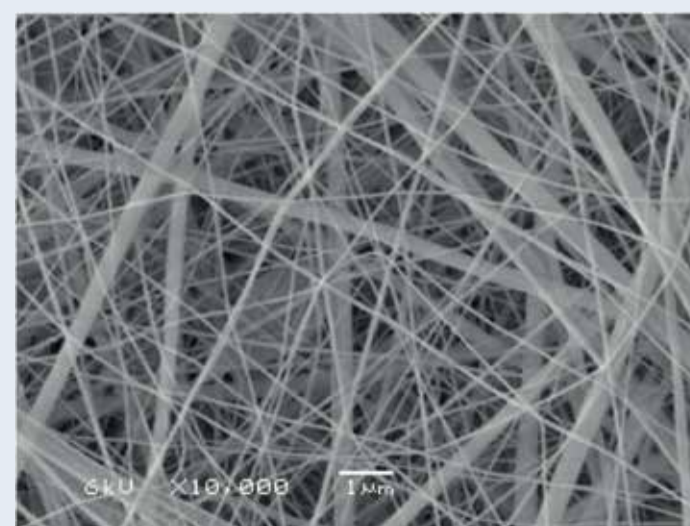
Fig 2. SEM image (10,000x magnification) of an electrospun interfacial layer, comprising fibers from 2 different polymers.
