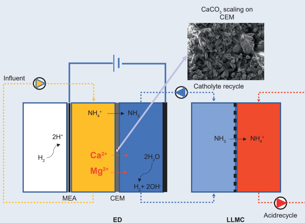
Figure 1. Inorganic scaling of CEM in ES ammonia recovery. MEA: membrane electrode assembly, CEM: cation exchange membrane, ED: electrodialysis, LLMC: liquid-liquid membrane contactor. Adapted from [4].
